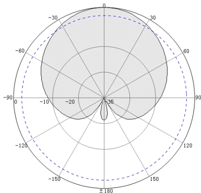
2450MHz- Horizontal Pattern
