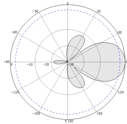
2450MHz- Vertical Pattern
