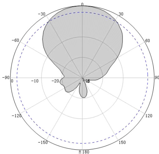
600MHz-Horizontal Pattern
