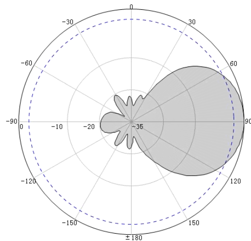
600MHz- Vertical Pattern
