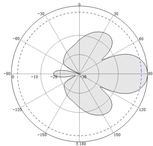
Vertical Pattern
