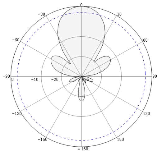
Horizontal Pattern
