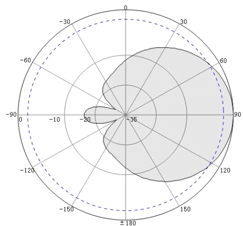
Vertical Pattern
