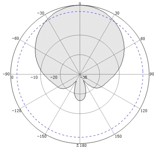
Horizontal Pattern
