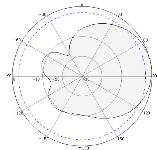
Vertical Pattern
