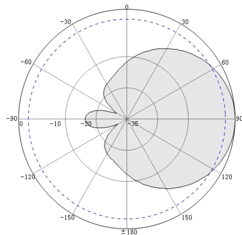
Vertical Pattern
