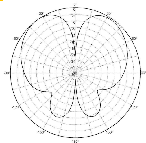
Vertical Pattern
