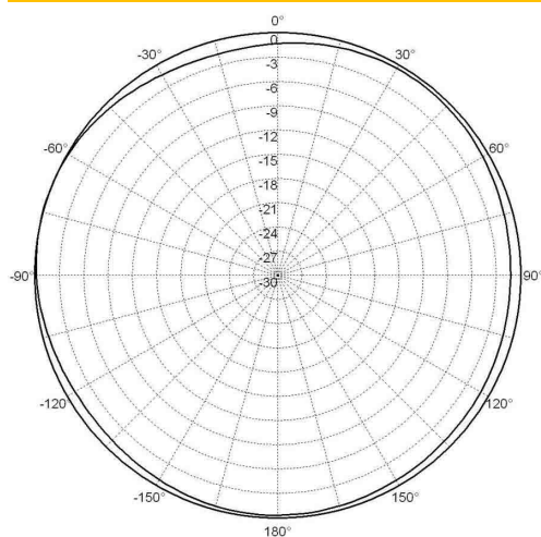
Horizontal Pattern
