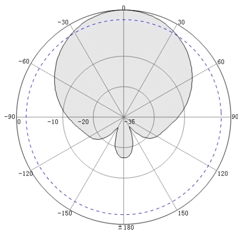
Horizontal Pattern
