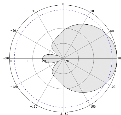
Vertical Pattern
